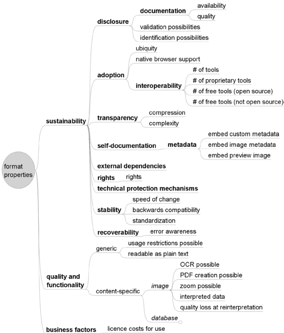
Figure 3 Format factors and associated criteria
