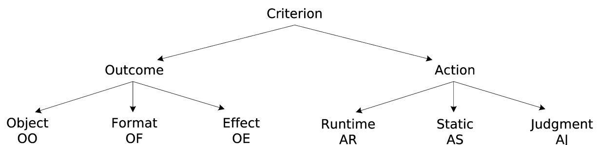
Figure 2 Generic criteria taxonomy
